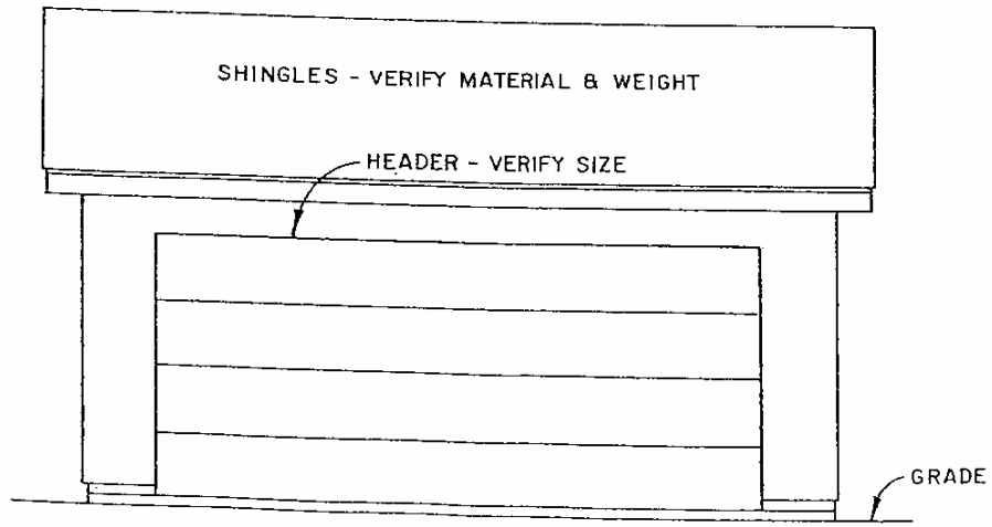
FRONT ELEVATION 1/4" = 1'-0"
